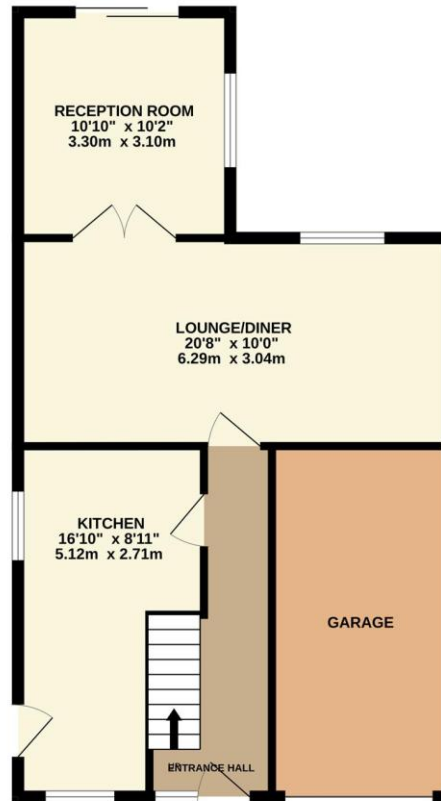
GROUND FLOOR 663 sq.ft. (61.6 sq.m.) approx.
